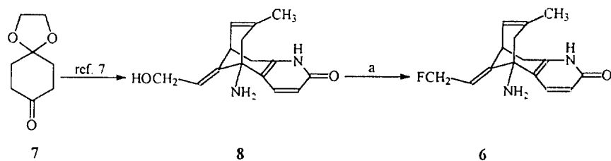
Scheme 1. Synthesis of (±)-14-fluorohuperzine A ( 6 )
